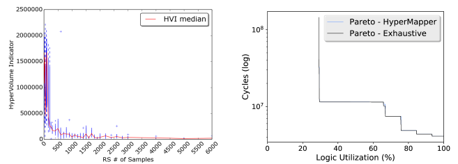
(a) HyperMapper HVI versus initial number of random samples ( R ) (b) Exhaustive and HyperMapper ( R=1000 ) generated Pareto curves.
